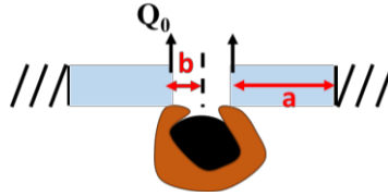
Fig.1 Schematic of the dried-longan pulp-peeling silicone plate, showing a central circular hole plate and a clamped (fixed) outer edge.
